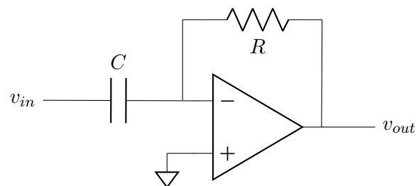
Figure 5: Ideal differentiator
