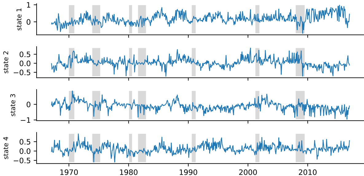
LSTM hidden macro states (trial 0); shaded = NBER recessions
