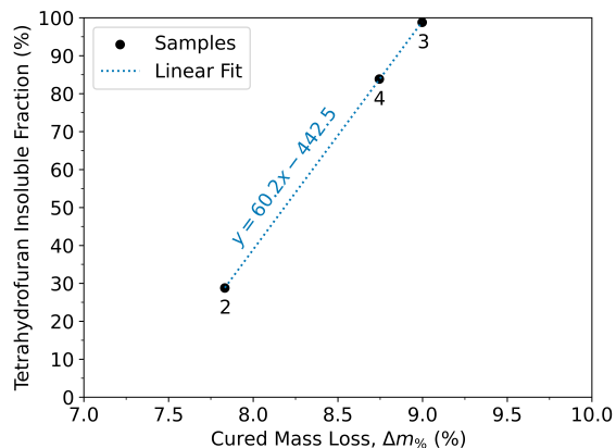
Figure 3: Overview of the relationship between the mass loss proxy variable and THF-insoluble fraction associated with a given formulation. Numbering indicates the 3 samples which were recoverable and characterised during the course of experimentation.
