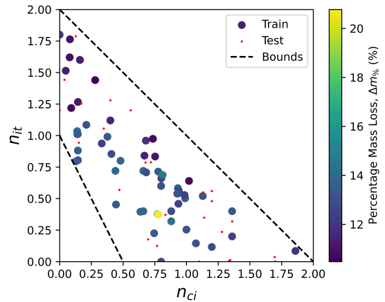
Figure 8: Overview of the test/train split undertaken with respect to the consolidated dataset. Bounds describe the outer edges of the parameter space.
