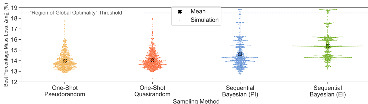
Figure 9: Swarm plot of maximum function evaluations obtained, \Delta m\% , for each of the 4,000 simulated optimisations carried out. All optimisations used 27 samples, each technique was simulated 1,000 times, and the Bayesian routines were initiated with 8 quasirandomly sampled points.
