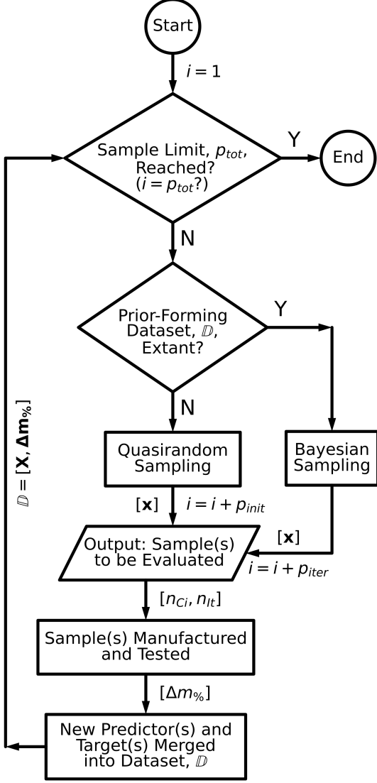
Figure 5: Flow diagram depicting the sequential optimisation algorithm developed.
