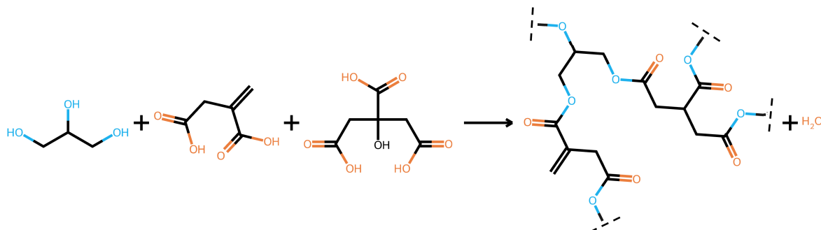
Figure 2: Polyesterification between glycerol, citric acid, and itaconic acid forming poly(glycerol citrate itaconate). Functional groups participating in the reaction are highlighted: hydroxyl groups blue, and carboxyl groups orange. In the products, ester groups are blue and carbonyl groups and water are orange in accordance with provenance.
