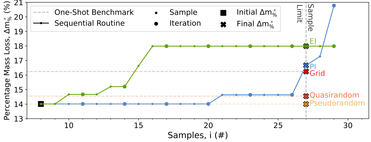
Figure 8: A plot comparing the optimisation progression for the two Bayesian sequential techniques alongside the three one-shot benchmark techniques. Expected improvement (EI) - solid green line. Probability of improvement (PI) - solid blue line. One-shot techniques - dashed lines. Uncertainty in \Delta m_{\%} values is equal to 0.44% points ( 1\sigma ).
