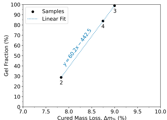
Figure 3: Overview of the relationship between the mass loss proxy variable and gel fraction associated with a given formulation. Numbering indicates the 3 samples which were recoverable and characterised during the course of experimentation.
