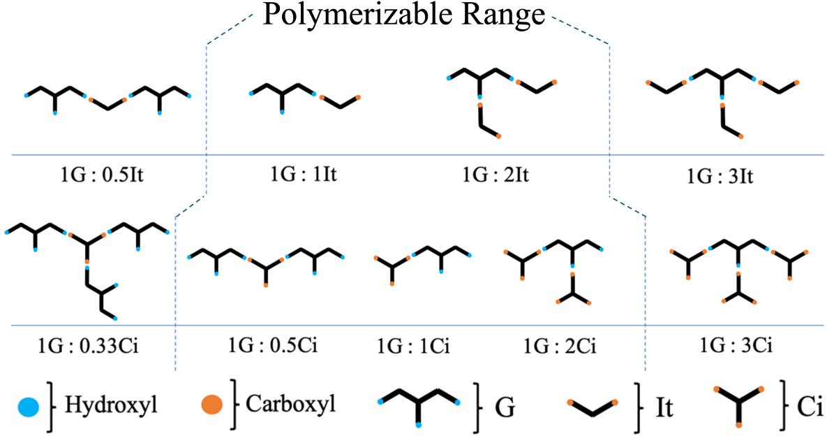
Figure 4: Simplified chemical representations displaying the polymerisable range of the two different triol-acid combinations encountered during poly(glycerol itaconate) synthesis. These ranges represent the stoichiometric intervals where di-functional and trifunctional monomers allow network formation; outside these bounds gelation may not occur. In the legend: “G” glycerol, “It” itaconic acid, ‘Ci’ citric acid.
