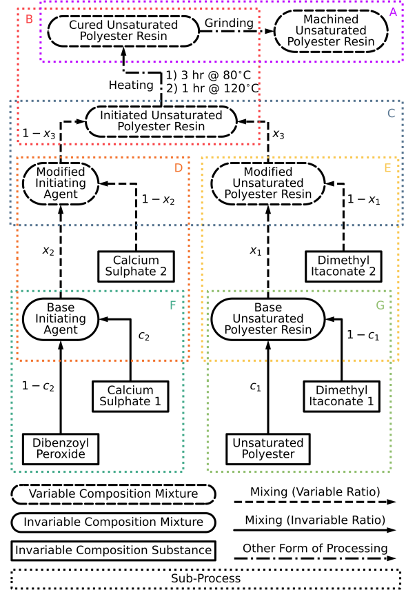
Figure 6: Mixing and processing schedule for the manufacture of thermoset composite samples. (A) Machining. (B) Thermochemical curing. (C) Mixing for initiated sample. (D) Mixing for modified initiator. (E) Mixing for modified resin. (F) Manufacturer's mixing for base initiator. (G) In-house mixing for base resin.
