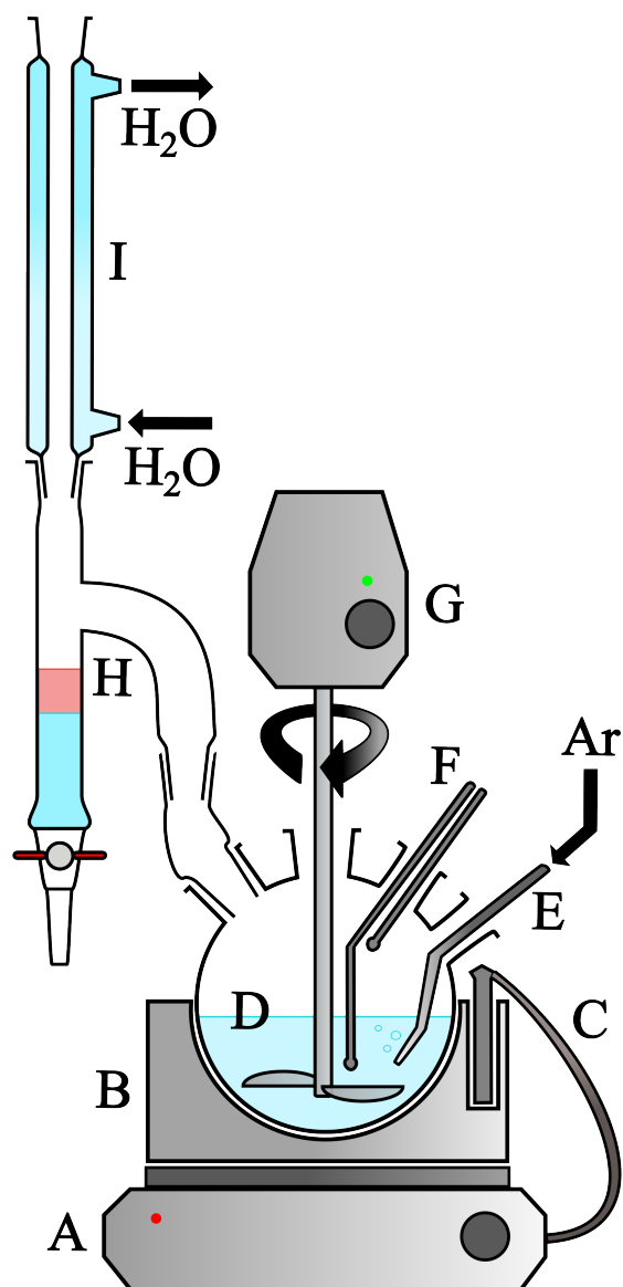
Figure 5: Apparatus for synthesis of unsaturated poly(propyl itaconate). (A) Hotplate stirrer (B) Aluminium bowl (C) Temperature controller probe (D) Four-necked round-bottomed flask containing the reaction mixture (E) Stainless-steel argon injector (F) Probes for batch and vapour temperatures (G) Overhead stirrer (H) Dean-Stark trap (I) Liebig condenser.
