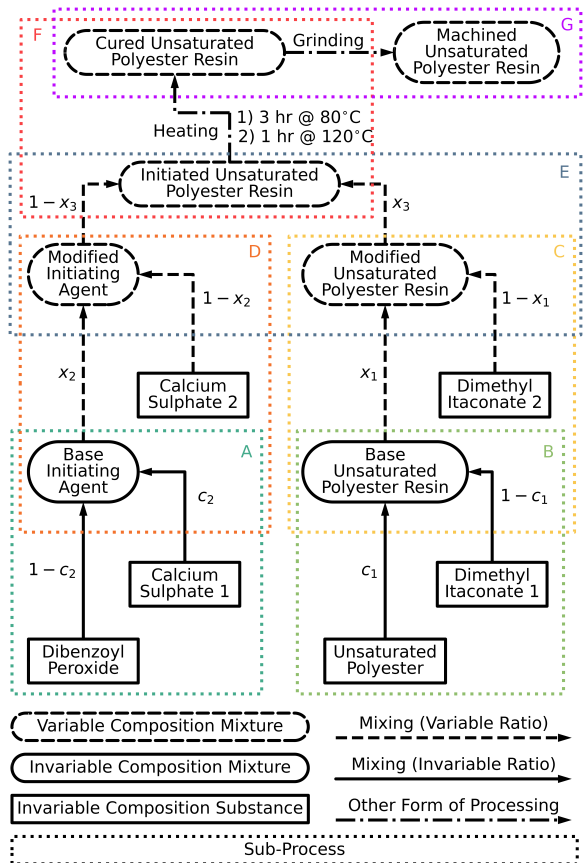
Figure 5: Mixing and processing schedule for the manufacture of thermoset composite samples. (A) Manufacturer’s mixing for base initiator. (B) In-house mixing for base resin. (C) Mixing for modified resin. (D) Mixing for modified initiator. (E) Mixing for initiated sample. (F) Thermochemical curing. (G) Machining.
