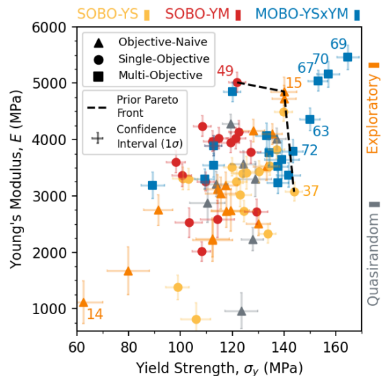
Figure 13: Multi-Objective Bayesian optimisation routine and results.
