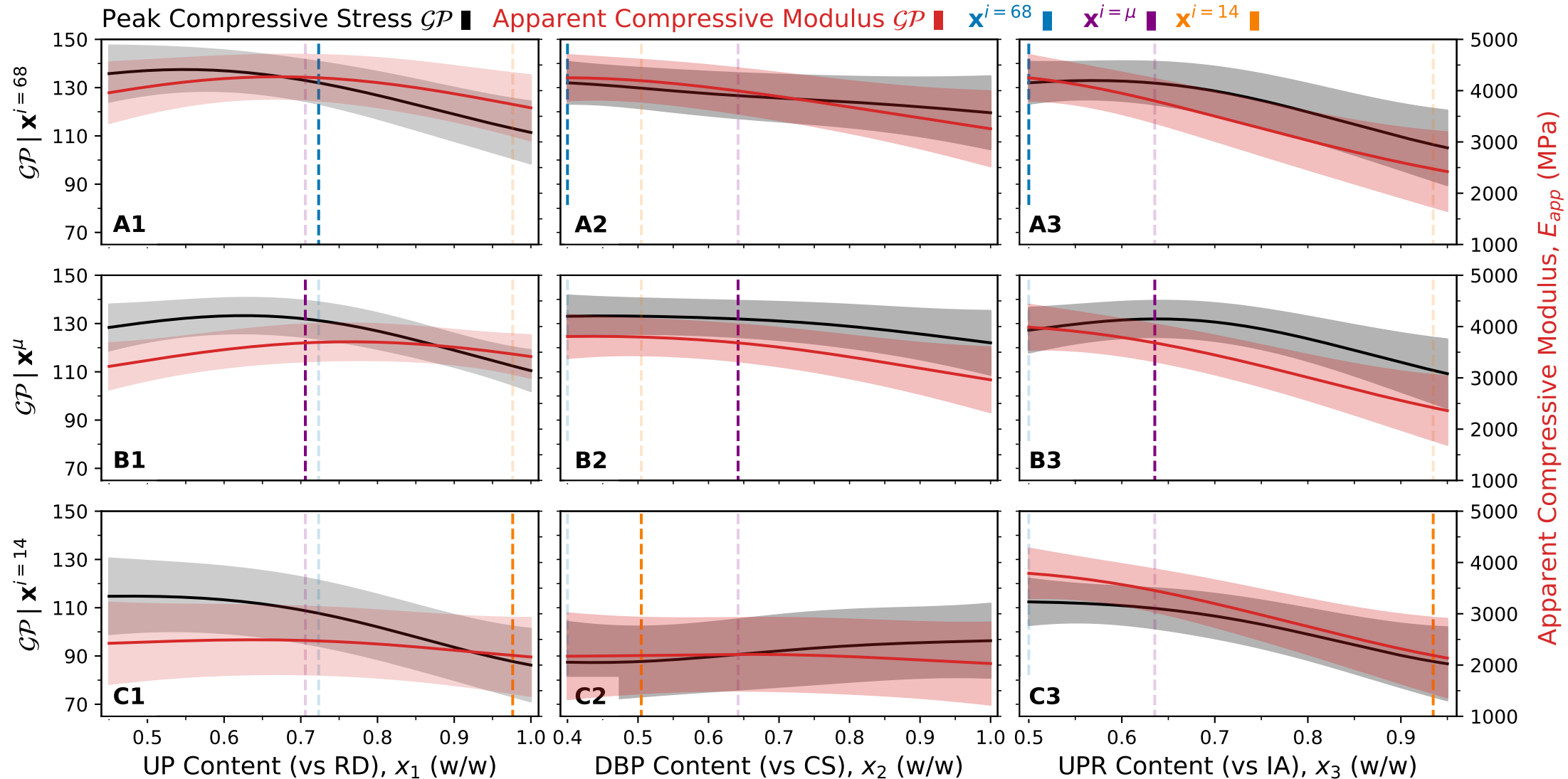
Peak Compressive Stress, \sigma_{max} (MPa)
