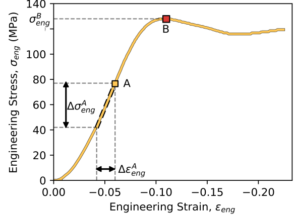
Figure 8: Automatic determination of apparent compressive modulus and peak compressive stress. (A) First inflection point. (B) Second inflection point.
