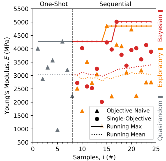
Figure 11: Progression of a sequential optimisation experiment concerning the maximisation of Young’s modulus.
