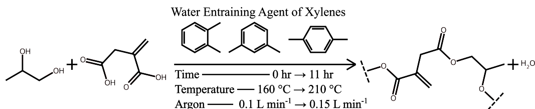
Figure 4: Simple reaction scheme for synthesis of poly(propylene itaconate).
