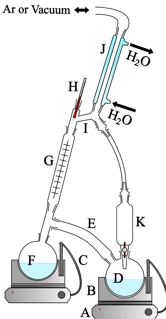
Figure 2: Apparatus for synthesis of dimethyl itaconate. (A) Hotplate stirrer (B) Aluminium bowl (C) Temperature controller probe (D) Three-necked round-bottomed flask containing the reaction mixture (E) Insulated glass tube (F) Single-necked round-bottomed flask acting as a distillation column reboiler containing water (G) Distillation column (H) Thermometer (I) Four-way Claisen head (J) Liebig condenser (K) Dropping funnel for recycled methanol
