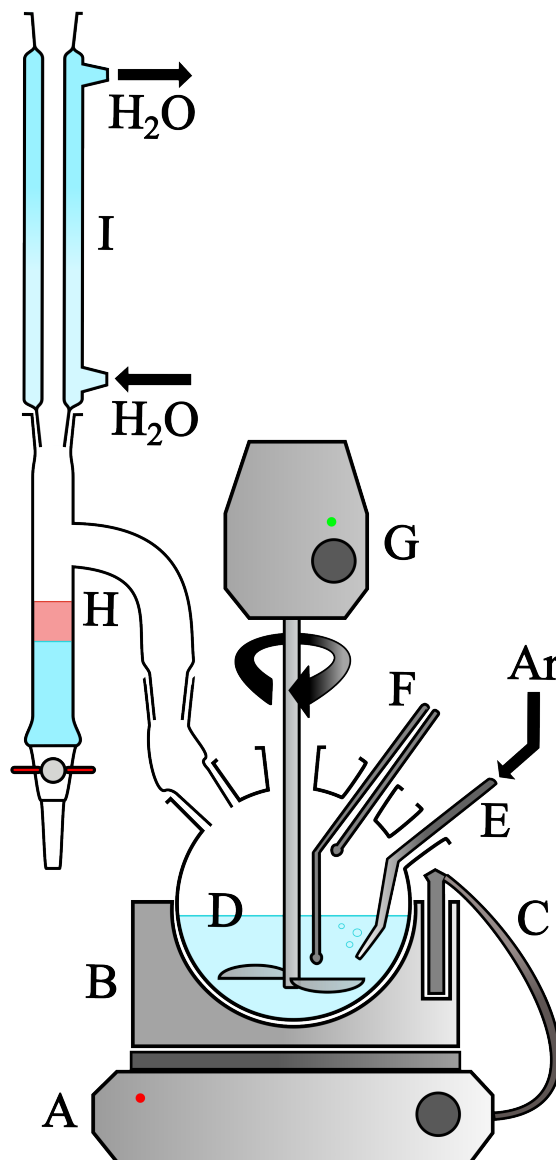
Figure 5: Apparatus for synthesis of unsaturated poly(propyl itaconate). (A) Hotplate stirrer (B) Aluminium bowl (C) Temperature controller probe (D) Four-necked round-bottomed flask containing the reaction mixture (E) Stainless-steel argon injector (F) Probes for batch and vapour temperatures (G) Overhead stirrer (H) Dean-Stark trap (I) Liebig condenser.
