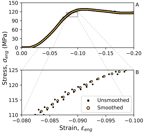
Figure 8: Multi-scale depiction of the stress-strain dataset before and after downscaling. (A) Overview line plot. (B) Zoomed scatter plot.
