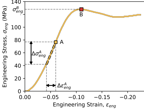
Figure 10: Means by which Young’s modulus and yield point were acquired from an archetypical stress-strain dataset. (A) First inflection point. (B) Second inflection point.
