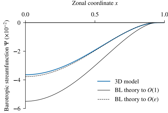
FIG. 8. Comparison of the barotropic streamfunction \Psi at t = 10^{-2} and y = 0 between the 3D f -plane inversion and the local model assuming along-slope symmetry (40). The modifications to the local model described in appendix C are applied to partially account for the added viscous terms in the 3D model.
