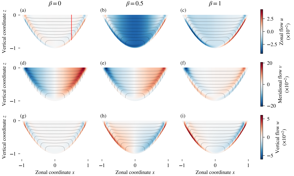
FIG. 4. Zonal sections at y = 0 of velocity components (colors) and isopycnals (gray lines) at t = 10^{-2} for (column 1; a, d, g) \beta = 0 , (column 2; b, e, h) \beta = 0.5 , and (column 3; c, f, i) \beta = 1 . The velocity components are organized by row, with (row 1; a, b, c) zonal flow u at the top, (row 2; d, e, f) meridional flow v in the middle, and (row 3; g, h, i) vertical flow w at the bottom. The red line in (a) indicates the location of profiles in Fig. 5.
