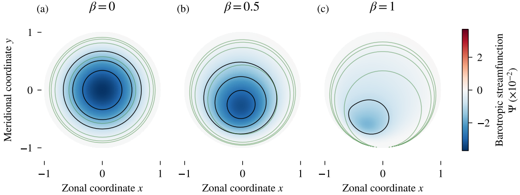
FIG. 6. Barotropic streamfunction \Psi (colors and black contours) at t = 10^{-2} for (a) \beta = 0 , (b) \beta = 0.5 , and (c) \beta = 1 . Negative values imply counter-clockwise flow. For reference, the f/H contours from Fig. 3 are overlaid in green.
