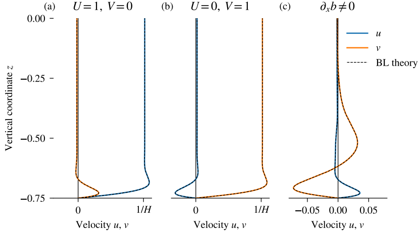
FIG. 7. Solutions to the frictional thermal wind equations (21) and (22) for cases with (a) zonal transport only (b) meridional transport only, and (c) no transport with a zonal buoyancy gradient taken from the bowl simulation at x = 0.5 , y = 0 , and t = 10^{-2} (see Fig. 1). Second-order accurate BL theory solutions (see appendix B) are shown in black dashed lines. Parameters are as in the full inversion at x = 0.5 and y = 0 ( \varepsilon = 2 \times 10^{-2} , f = 1 , \nu = 1 , H = 0.75 ) with horizontal viscous terms ignored.
