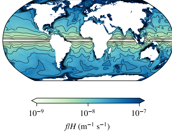
FIG. 2. Contours of f/H for the global ocean using bathymetry data from Smith and Sandwell (1997, updated). The data is smoothed by averaging over a 500 km diameter circle at each point.
