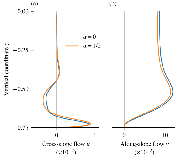
FIG. A1. Snapshot of (a) cross-slope flow u and (b) along-slope flow v satisfying the transport-constrained 1D equations (A8) to (A10) for aspect ratios \alpha = 0 and 1/2 and the same mixing-driven buoyancy field at t = 10^{-2} used in the main text. The column depth H = 0.75 and local slope \theta = \pi/4 corresponding to the point x = 0.5 and y = 0 on the bowl, as in Fig. 5. In this case, the vertical velocity profile is the same as the cross-slope flow because w = u \tan \theta .
