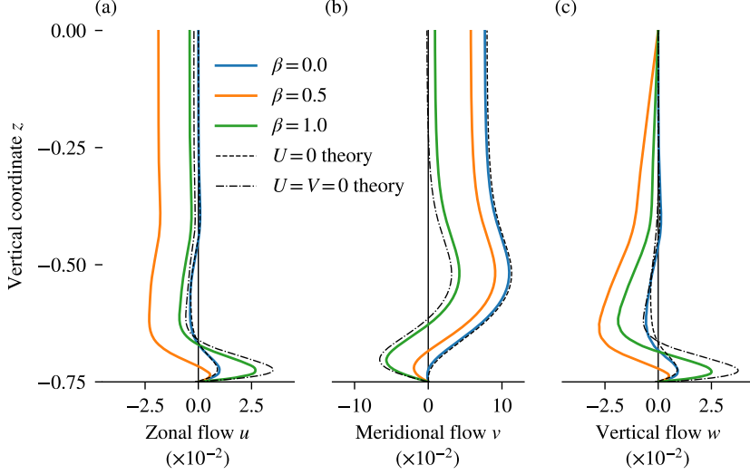
FIG. 5. Vertical profiles of (a) zonal u , (b) meridional v , and (c) vertical w flow components from the 3D model inversion (solid) for \beta = 0, 0.5, 1 at x = 0.5 , y = 0 , and t = 10^{-2} . The second-order accurate local models for U = 0 and U = V = 0 (modified for an aspect ratio of 1/2 , see appendices B and C) are shown in dashed and dashed-dotted lines, respectively.
