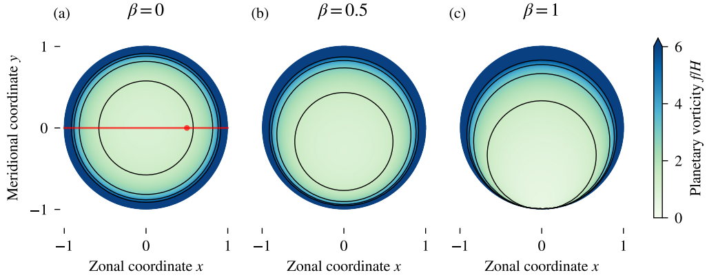
FIG. 3. Contours of f/H in a circular mid-latitude basin for H = 1 - x^2 - y^2 and (a) f = 1 , (b) f = 1 + 0.5y , (c) f = 1 + y . The red line and circle in (a) indicate where the zonal slices in Fig. 4 and the profiles in Fig. 5 are taken, respectively.
