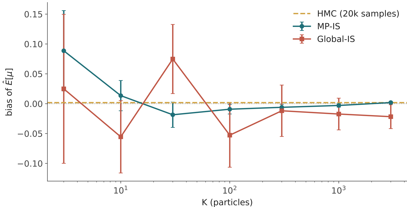
Self-normalization bias shrinks with K
