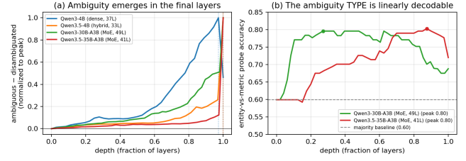
Figure 3: Four-model depth profile of the ambiguity signal (Qwen3 4B \rightarrow 35B, dense and MoE). (a) Ambiguous-disambiguated separation rises to a peak in the final layers of every model (dotted verticals mark per-model peaks; normalized for depth and magnitude). (b) The ambiguity type (entity vs. metric) is linearly decodable at 0.80 on both MoE models, well above the 0.60 majority baseline, peaking at different depths.
