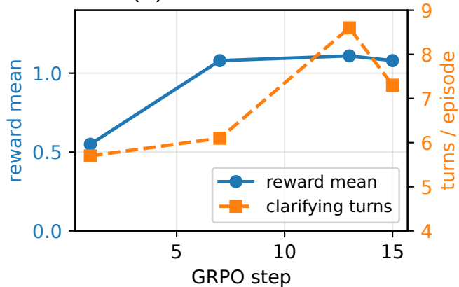
(b) Multi-turn GRPO
