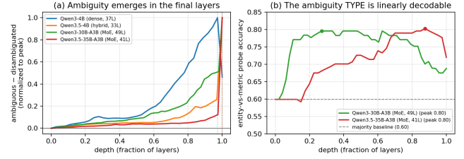
Figure 3: Four-model depth profile of the ambiguity signal (Qwen3 4B→35B, dense and MoE). (a) Ambiguous-disambiguated separation rises to a peak in the final layers of every model (dotted verticals mark per-model peaks; normalized for depth and magnitude). (b) The ambiguity type (entity vs. metric) is linearly decodable at 0.80 on both MoE models, well above the 0.60 majority baseline, peaking at different depths.
