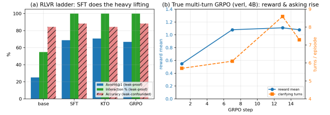
Figure 2: Training on FININTERACT. (a) The leak-proof learning signals (AxisHit@1, interaction) jump at SFT and saturate; accuracy (hatched) is leak-confounded. (b) True multi-turn GRPO on the 4B policy: mean reward and clarifying turns rise together over training.
