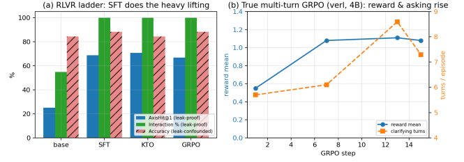
Figure 3: Training on FININTERACT. (a) The leak-proof learning signals (AxisHit@1, interaction) jump at SFT and saturate; accuracy (hatched) is leak-confounded. (b) True multi-turn GRPO on the 4B policy: mean reward and clarifying turns rise together over training.
