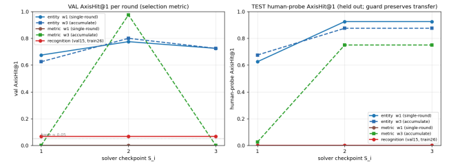
Figure 5: Multi-round co-evolution with a validation guard. Left : validation AxisHit@1 (selection metric) per round. Right : held-out human-probe AxisHit (never used for selection). Entity learns targeting from a single 30-instance slice and transfers to humans ( 0.63 \rightarrow 0.93 ); metric needs accumulation (one slice teaches nothing, brown, flat, while two accumulated slices reach 0.75, green); recognition stays at base ( \approx 0.05 ) even with a fair 26-instance set. The guard preserves human transfer (it rolls back the round-3 candidate, which regresses on validation).
