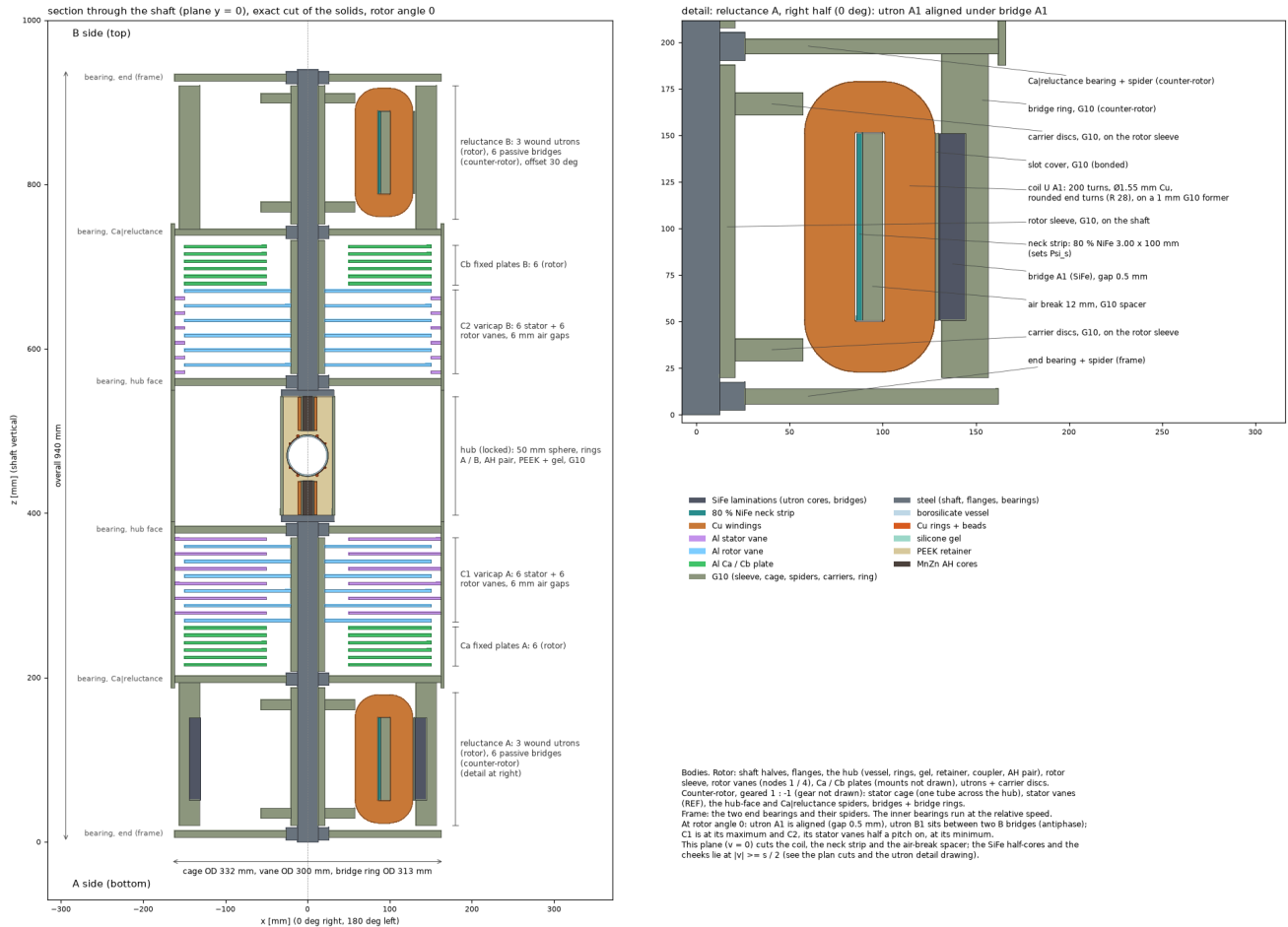
Figure 2. The machine of record in 3-D: the section through the shaft (side A below), with the air stack of record and Ca / Cb on the rotor, the reluctance sections and the locked hub; 940 mm. Source: docs/geometry/tube/tube-r150-n6-air6-wound-g0p5-6br-hub50-section.png (sim/tube_geometry.py --record).
