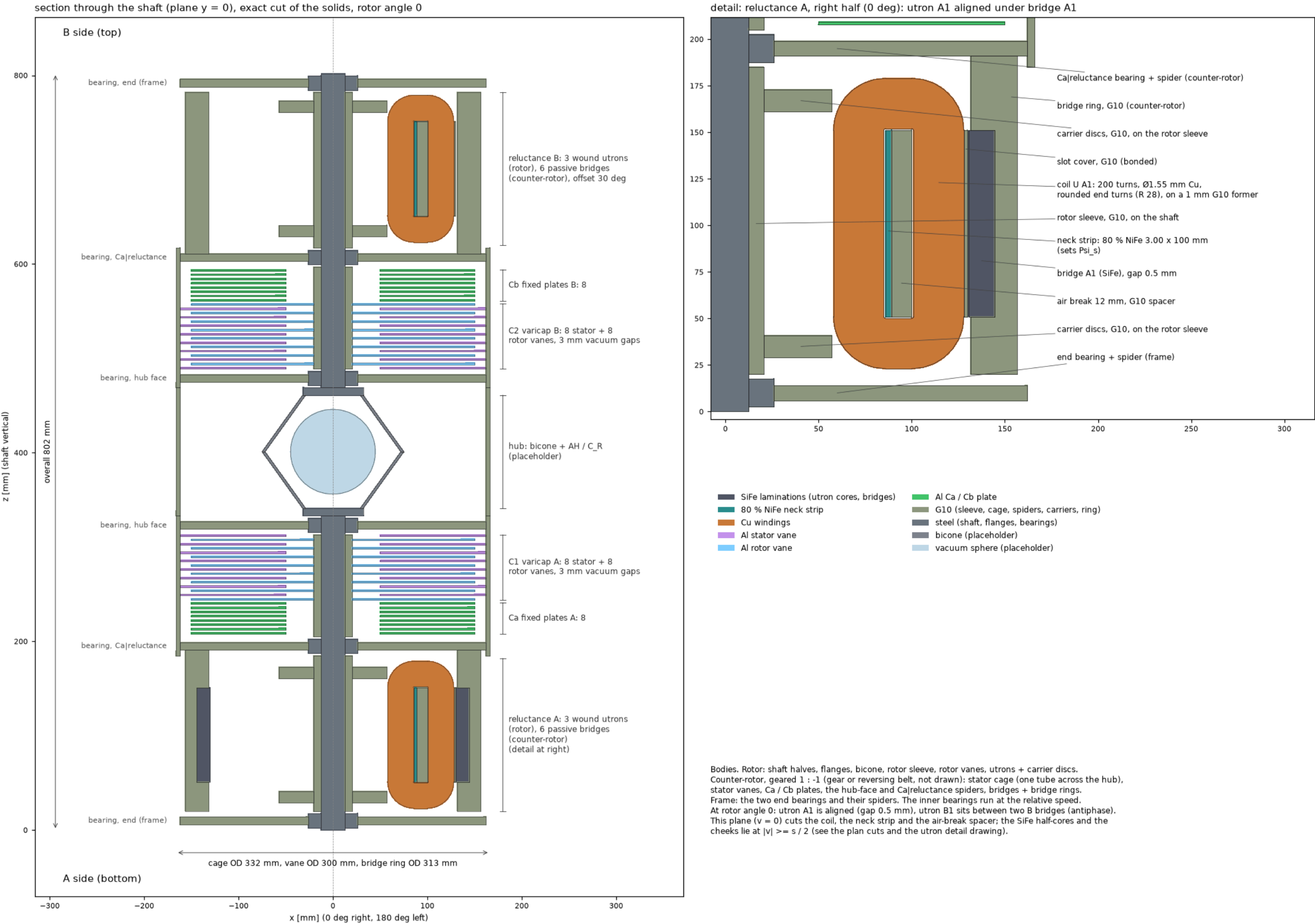
tube-r150-n8-wound-g0p5-6br: arrangement (g 0.5 / 6 bridges / 1200 rpm), 802 mm long
