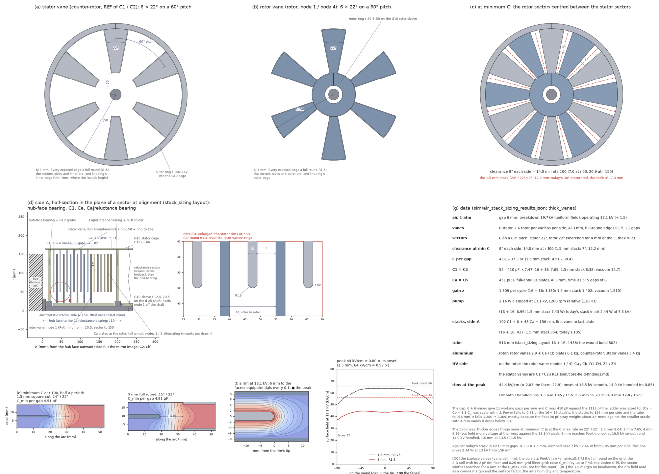
Figure 5. The air vane stack of record: the stator vane (REF), the rotor vane (node 1 / 4), both at minimum capacitance, side A's half-section, the vane cell and the rim field against Peek's onset. Panel (d) still draws the placeholder hub. Source: docs/figures/air-vane-stack-6mm.png ( docs/make_air_vane_drawing.py ).
