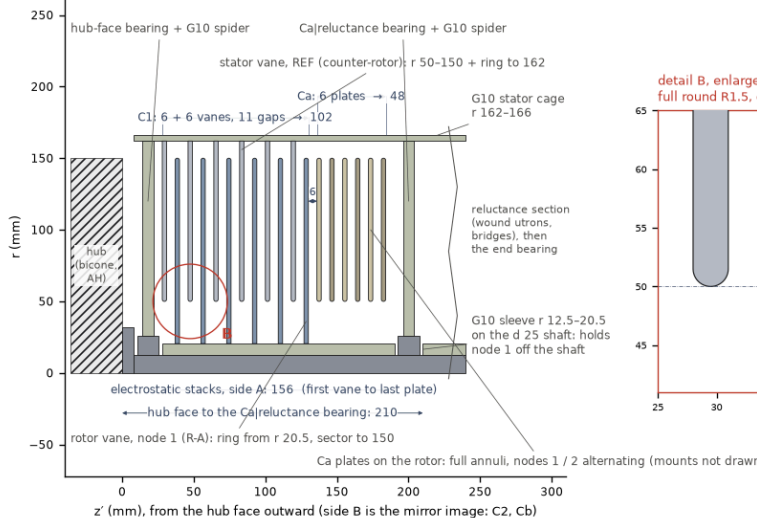
(d) side A, half-section in the plane of a sector at alignment (stack_sizing.layout): hub-face bearing, C1, Ca, Ca|reluctance bearing
