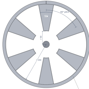
(a) stator vane (counter-rotor, REF of C1 / C2): 6 × 22° on a 60° pitch
