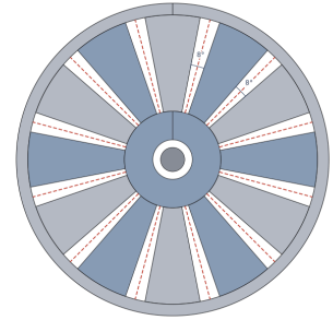
(c) at minimum C: the rotor sectors centred between the stator sectors
