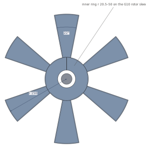
(b) rotor vane (rotor, node 1 / node 4): 6 × 22° on a 60° pitch
