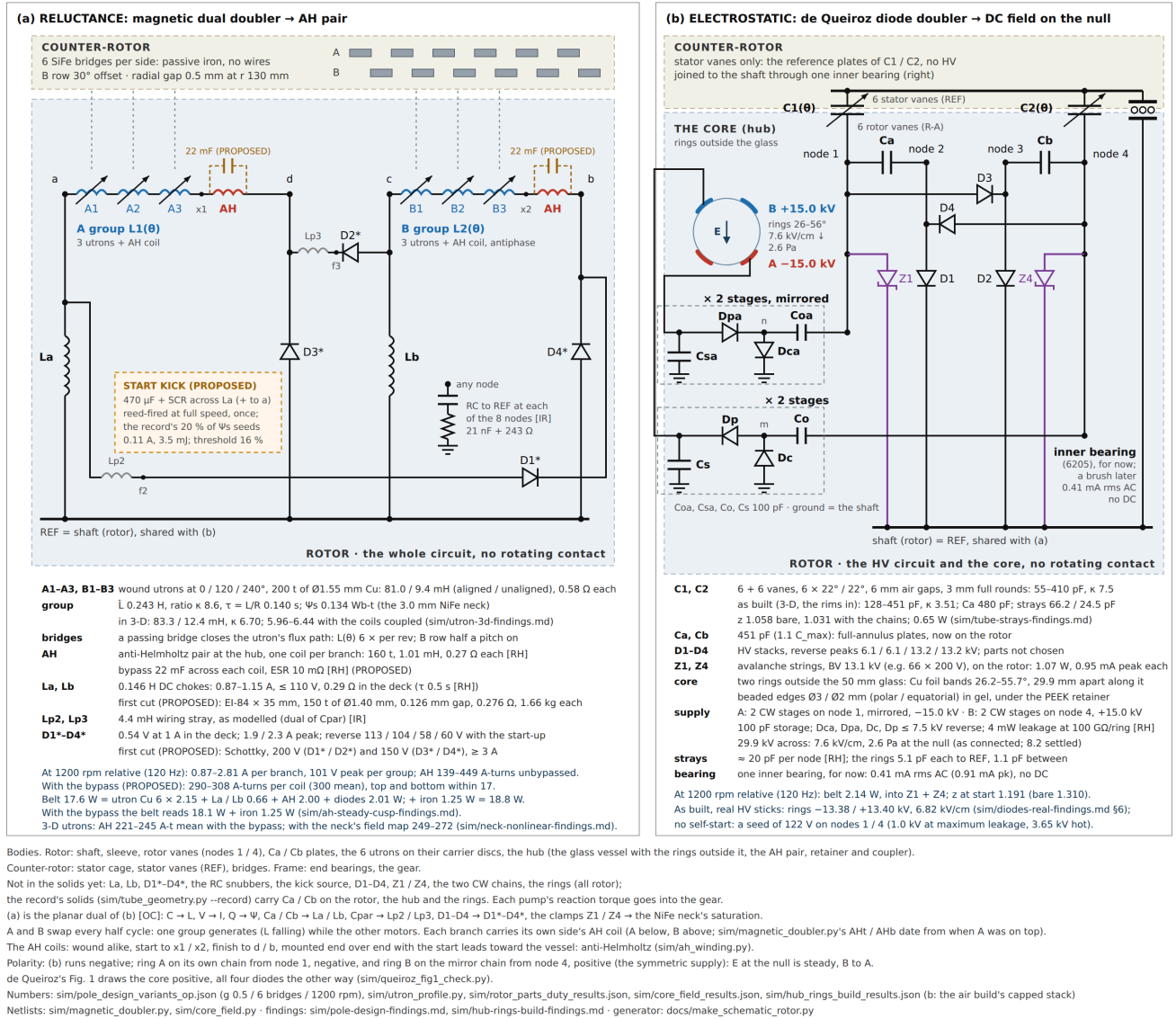
Figure 4. The rotor's two circuits as built: (a) the magnetic dual doubler driving the AH pair; (b) the electrostatic de Queiroz doubler with the HV side on the rotor and the rings' two mirrored chains. The 22 mF bypass across each AH coil is drawn dashed (PROPOSED). Source: docs/schematic-rotor-circuits.svg (docs/make_schematic_rotor.py).
