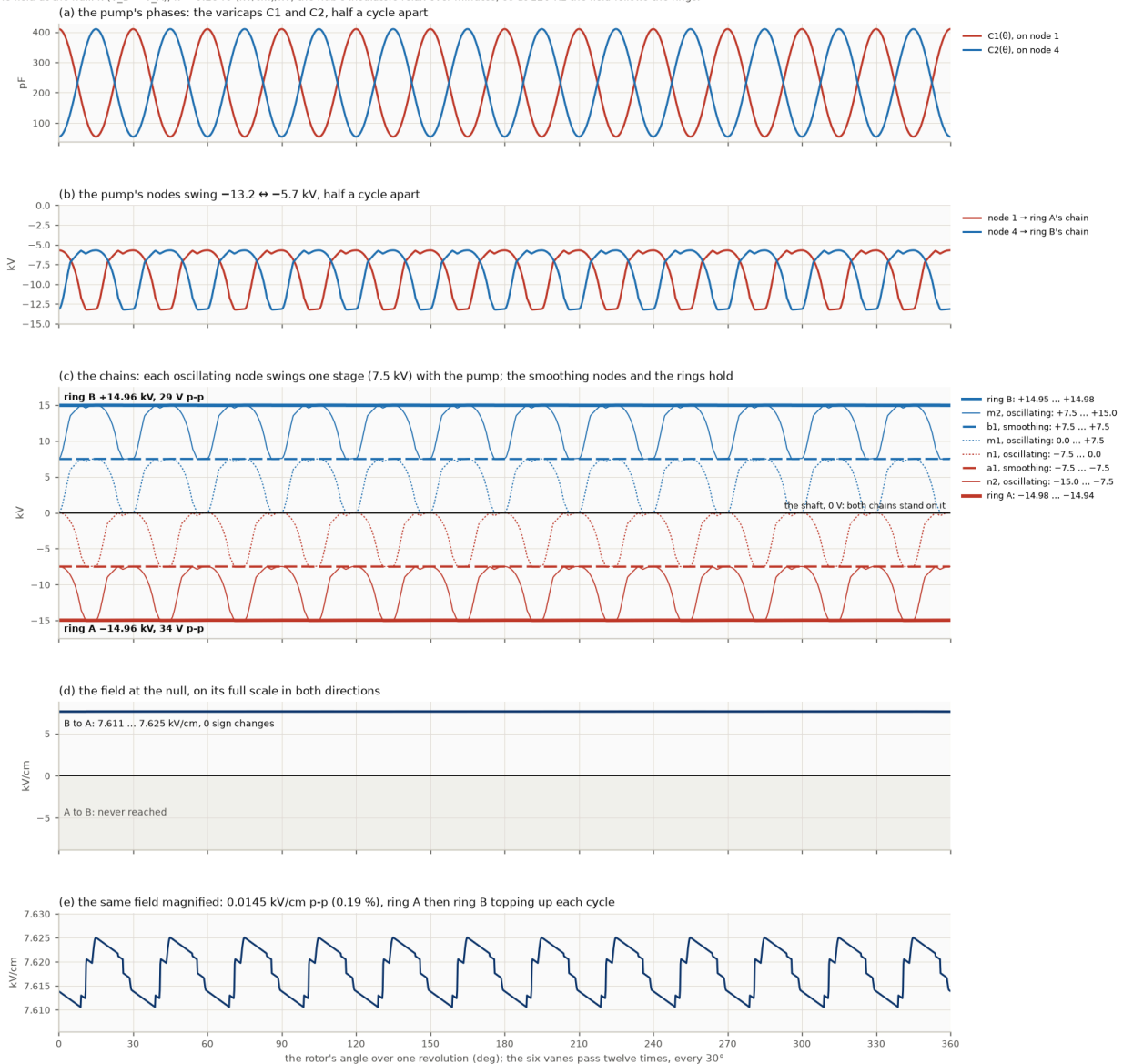
Figure 9. One revolution of the rotor: the pump goes through its phases twelve times (C1 / C2, nodes 1 / 4, the chains' oscillating nodes), while the rings hold and the field at the null stays 7.611–7.625 kV/cm from B to A. Source: docs/figures/hub-rings-revolution.png (sim/hub_revolution.py).
