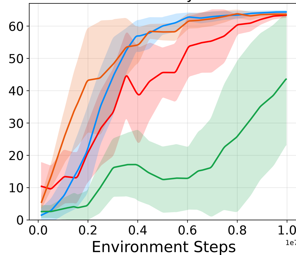
Freeway
