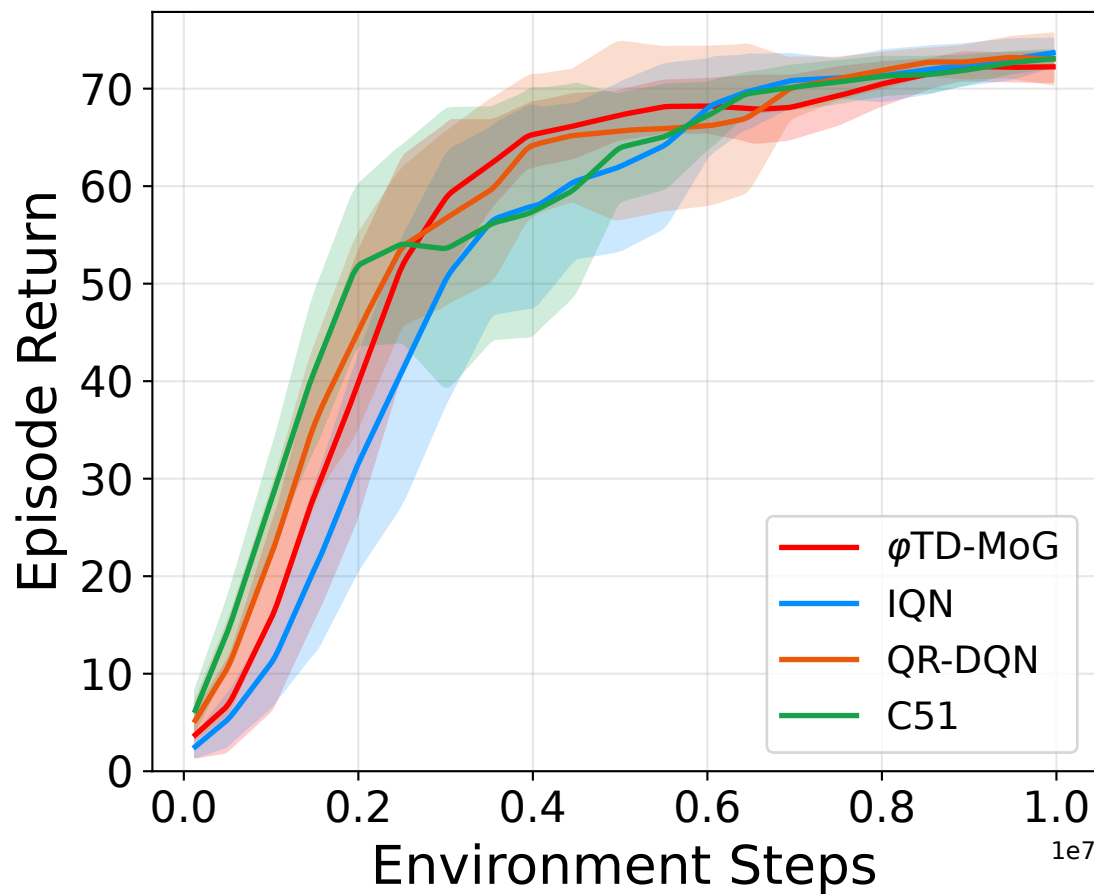
Asterix
