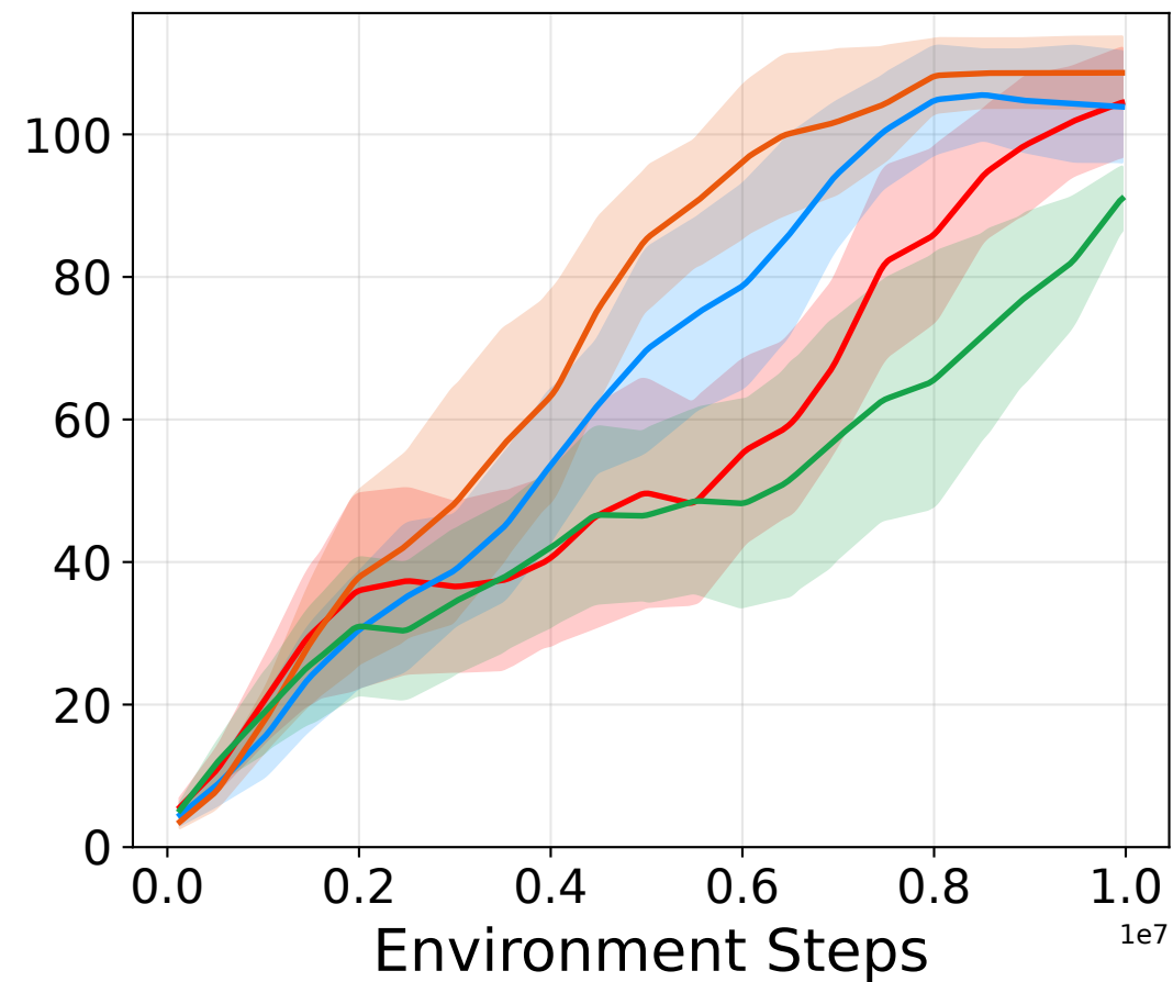
Breakout
