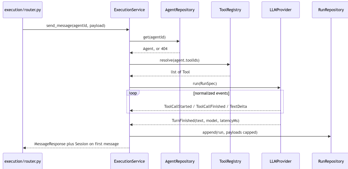
Figure 6: Agent execution flow
