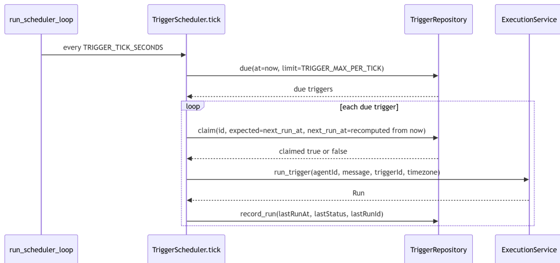
Figure 7: Trigger scheduler flow
