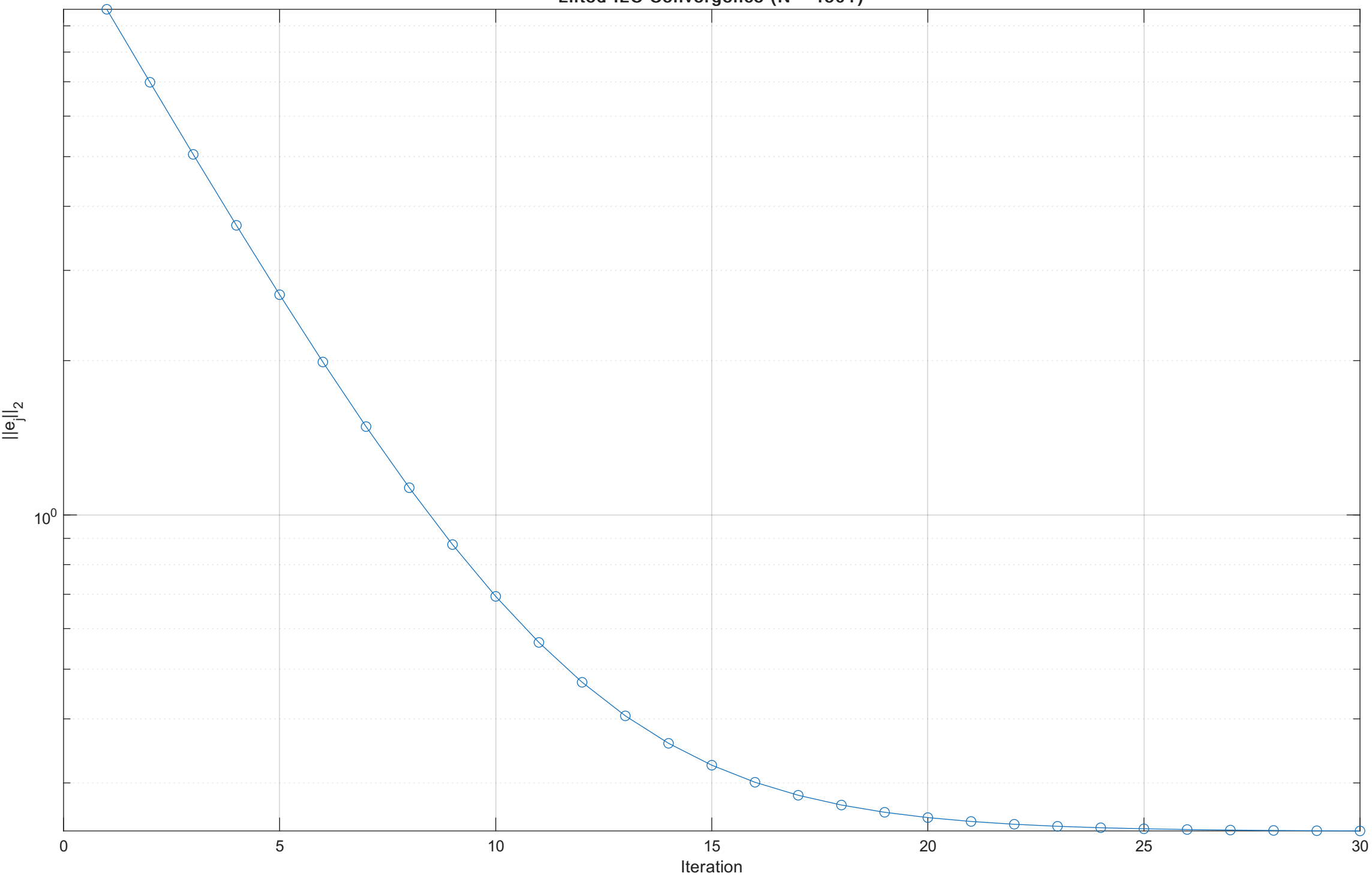
Lifted ILC Convergence (N = 4501)
