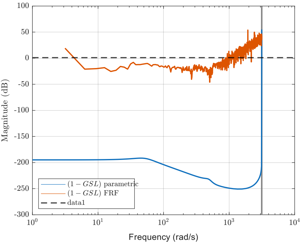
Bode Diagram
