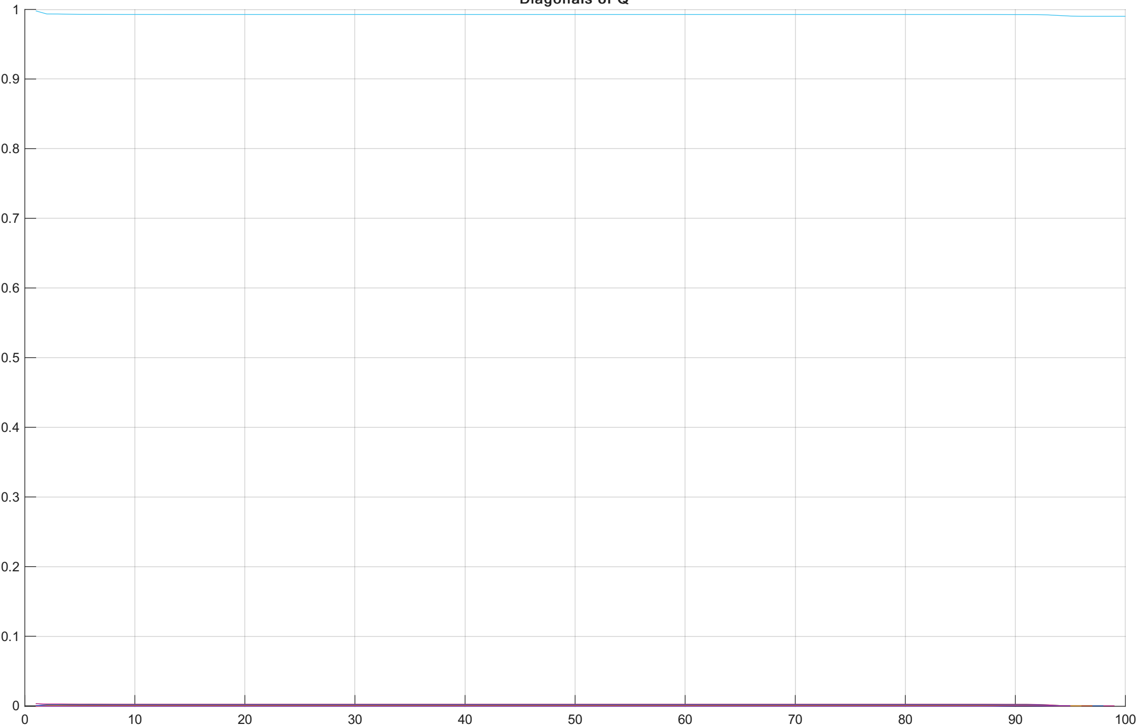
Diagonals of Q
