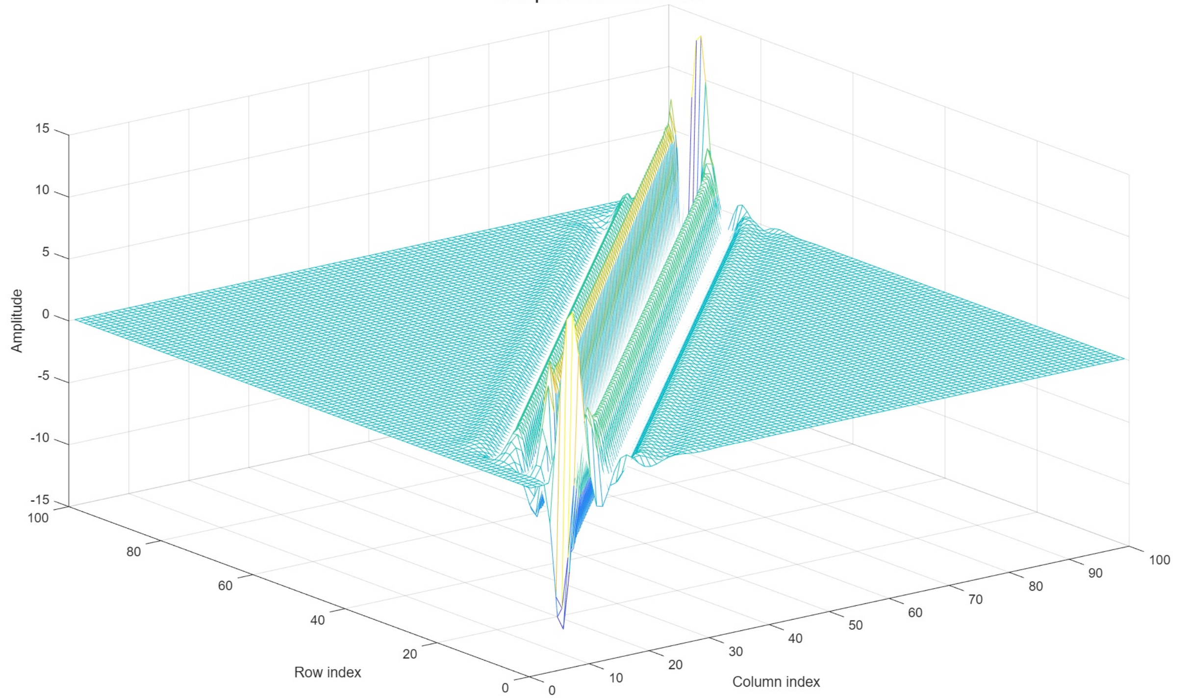
Mesh plot of lifted ILC matrix L
