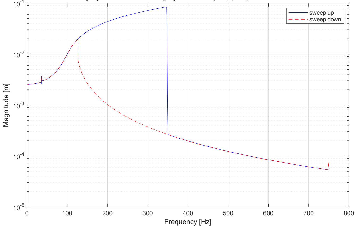
Sweep up and down of Duffing equation with f \in [1, 750] Hz and F = 469.5
