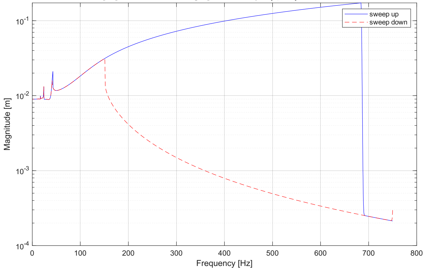
Sweep up and down of Duffing equation with f \in [1, 750] Hz and F = 1878
