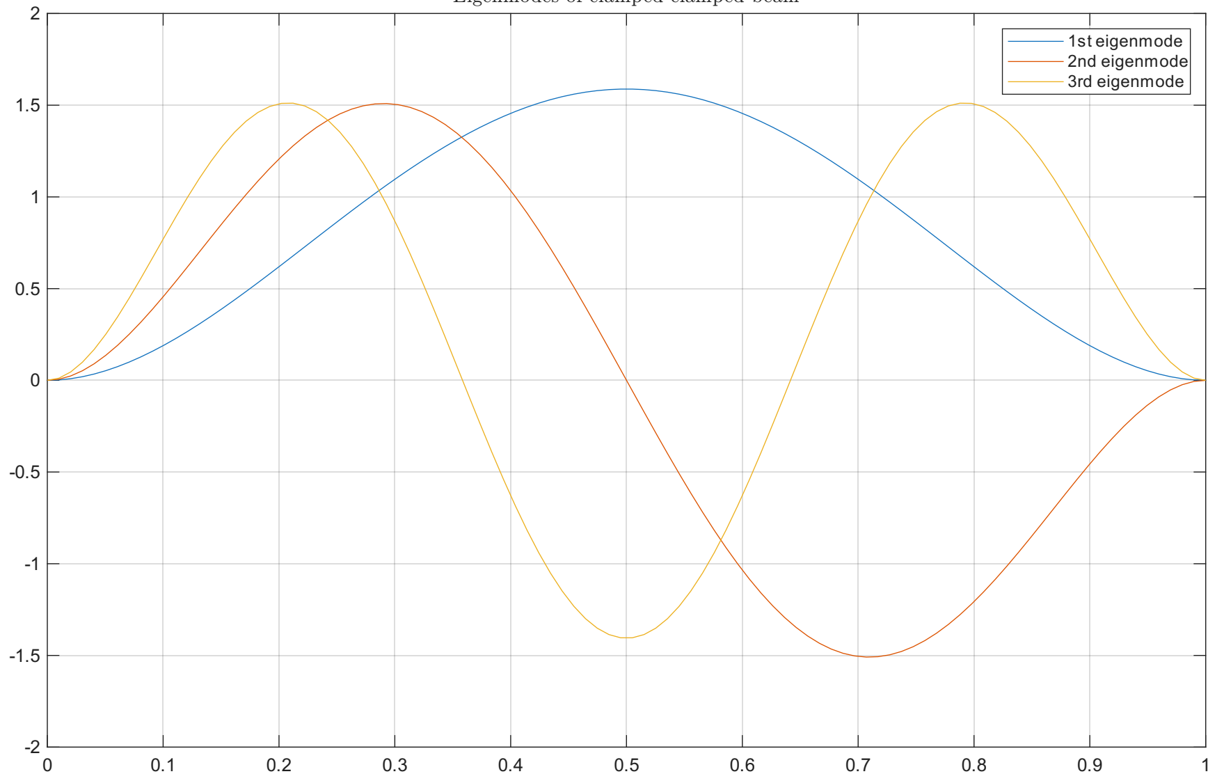
Eigenmodes of clamped clamped beam
