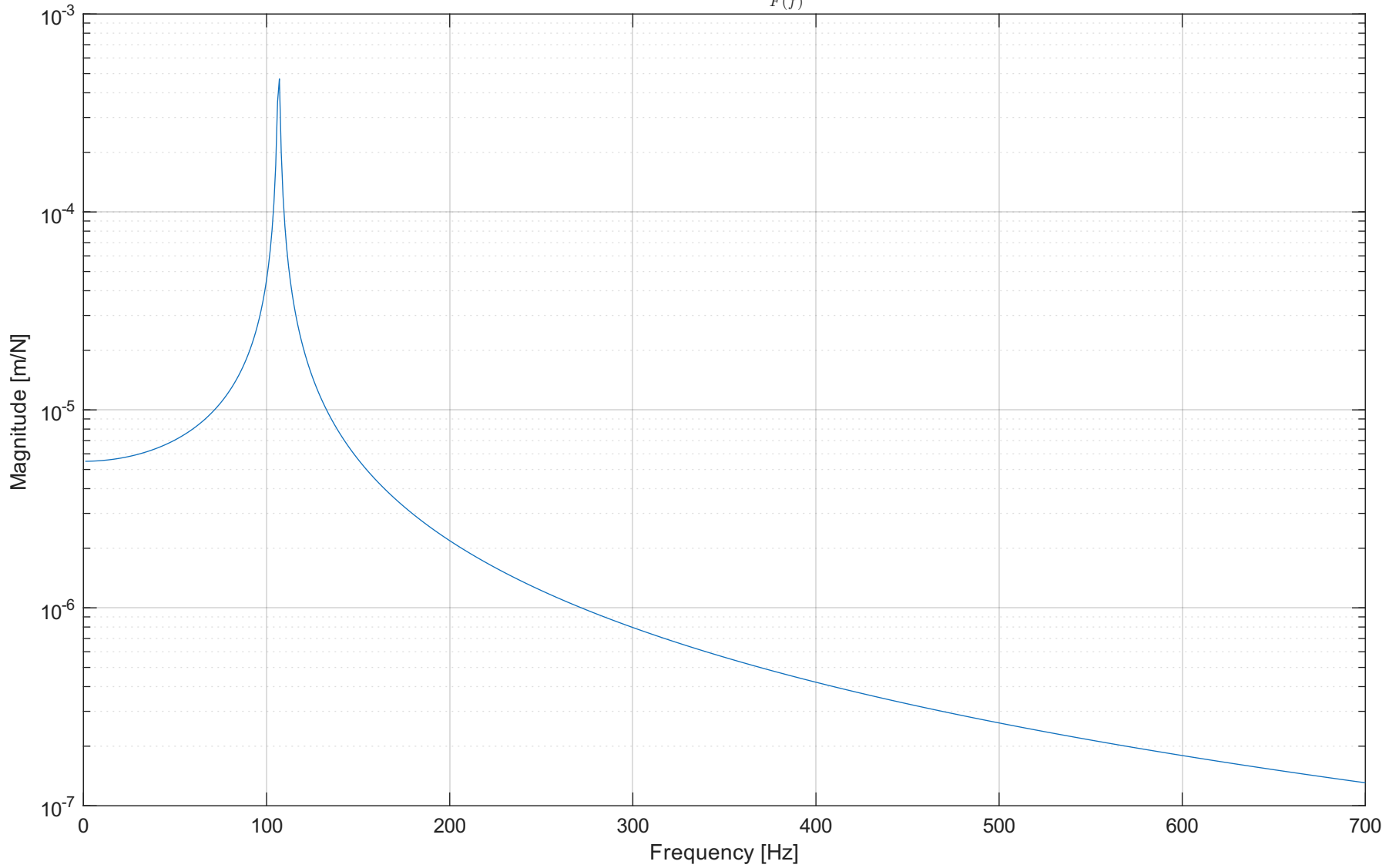
Linear FRF \frac{\hat{V}(\frac{L}{2}, f)}{\hat{F}(f)}
