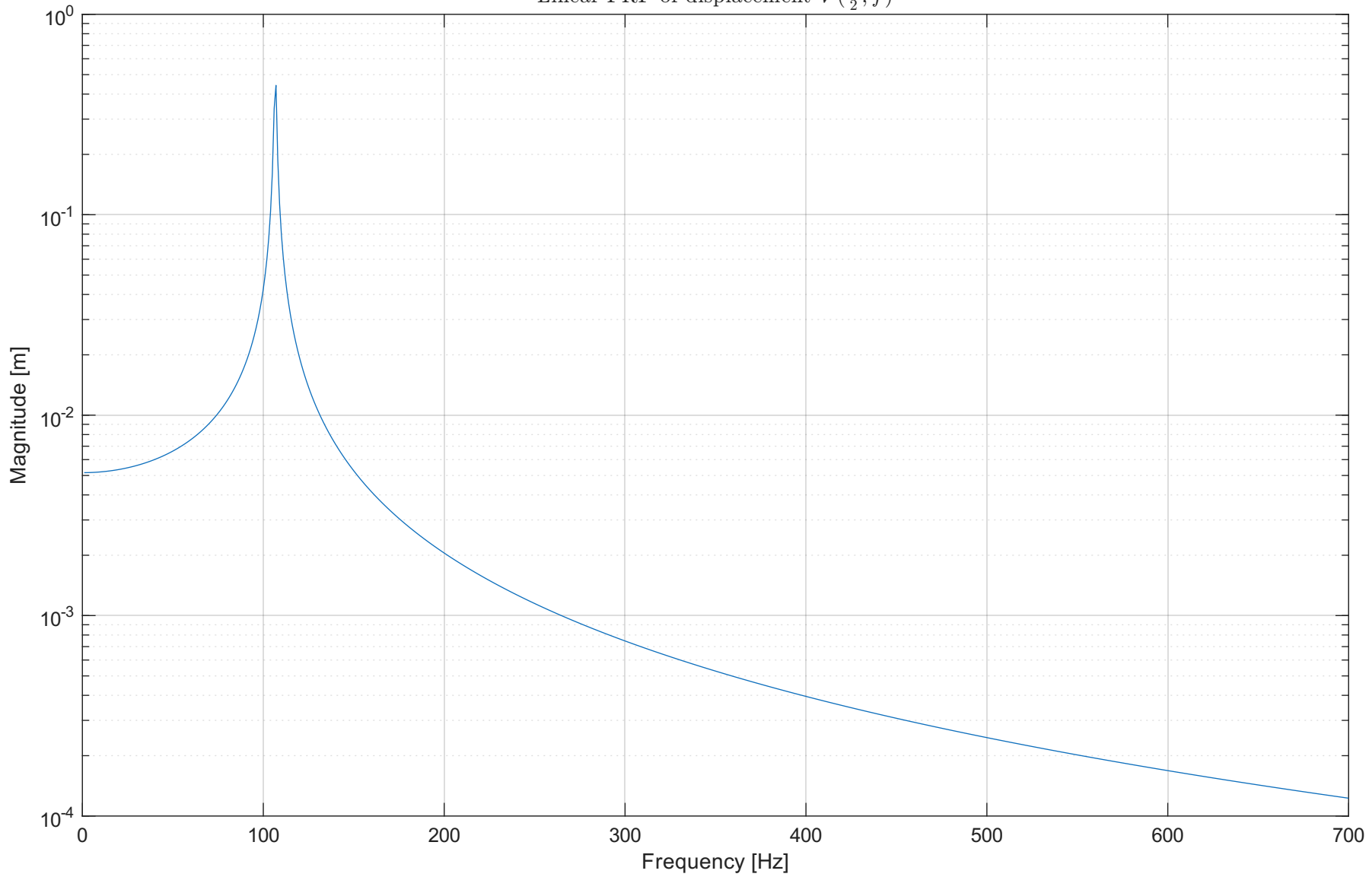
Linear FRF of displacement \hat{V}(\frac{L}{2}, f)
