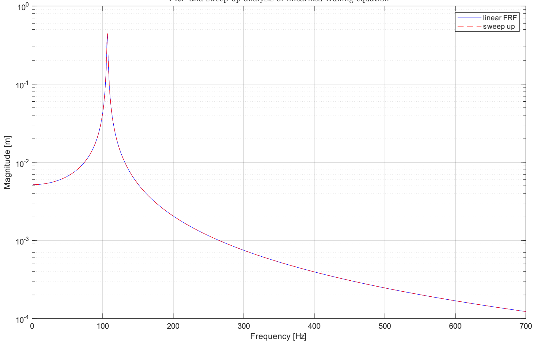
FRF and sweep up analysis of linearized Duffing equation
