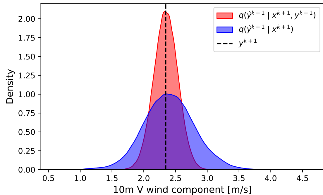
Posterior Predictive Check (PPC) for surface variables at lat=50, lon=5 (Europe)
