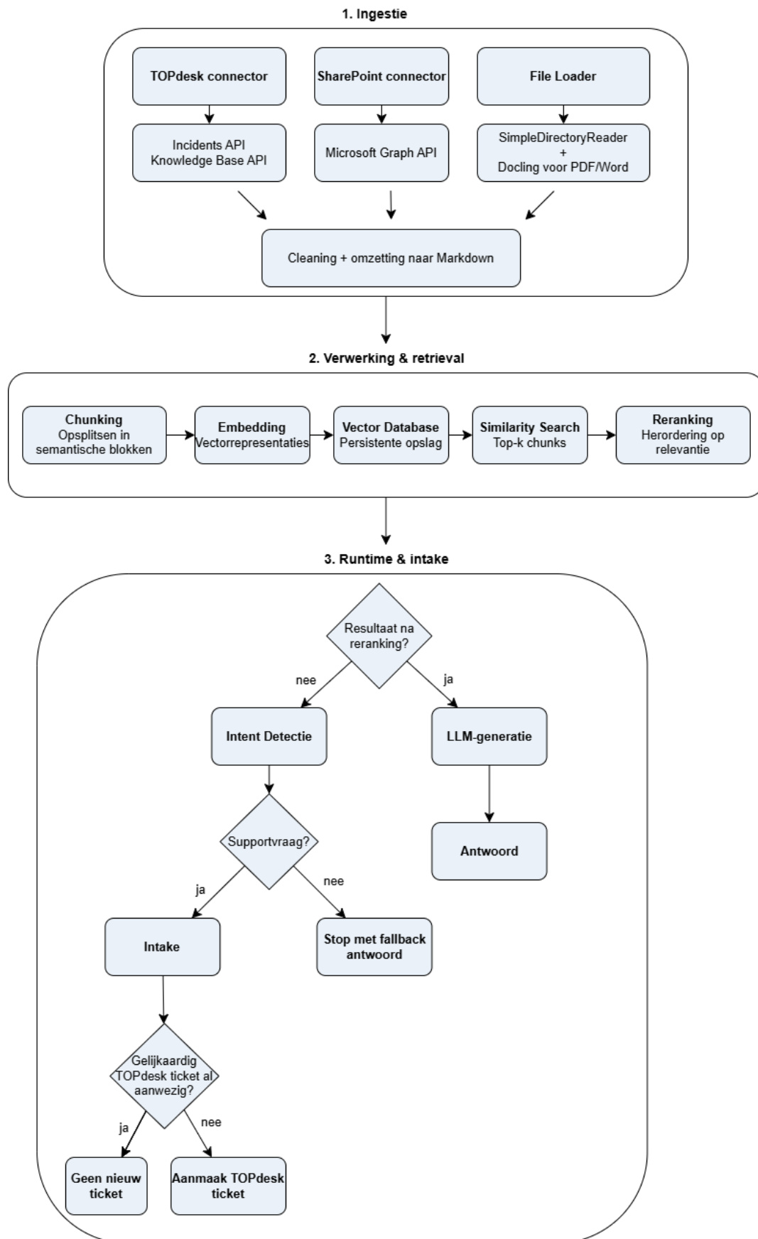
Figuur 4: Backend pipeline
