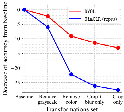
(b) Impact of progressively removing transformations
