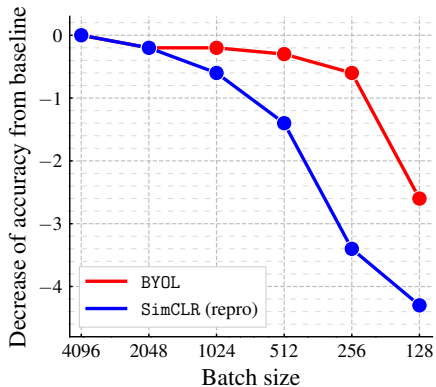
(a) Impact of batch size
