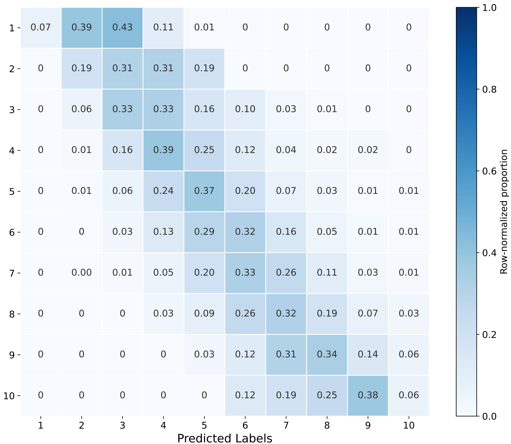
Normalized RPE Prediction Without EMG Features
