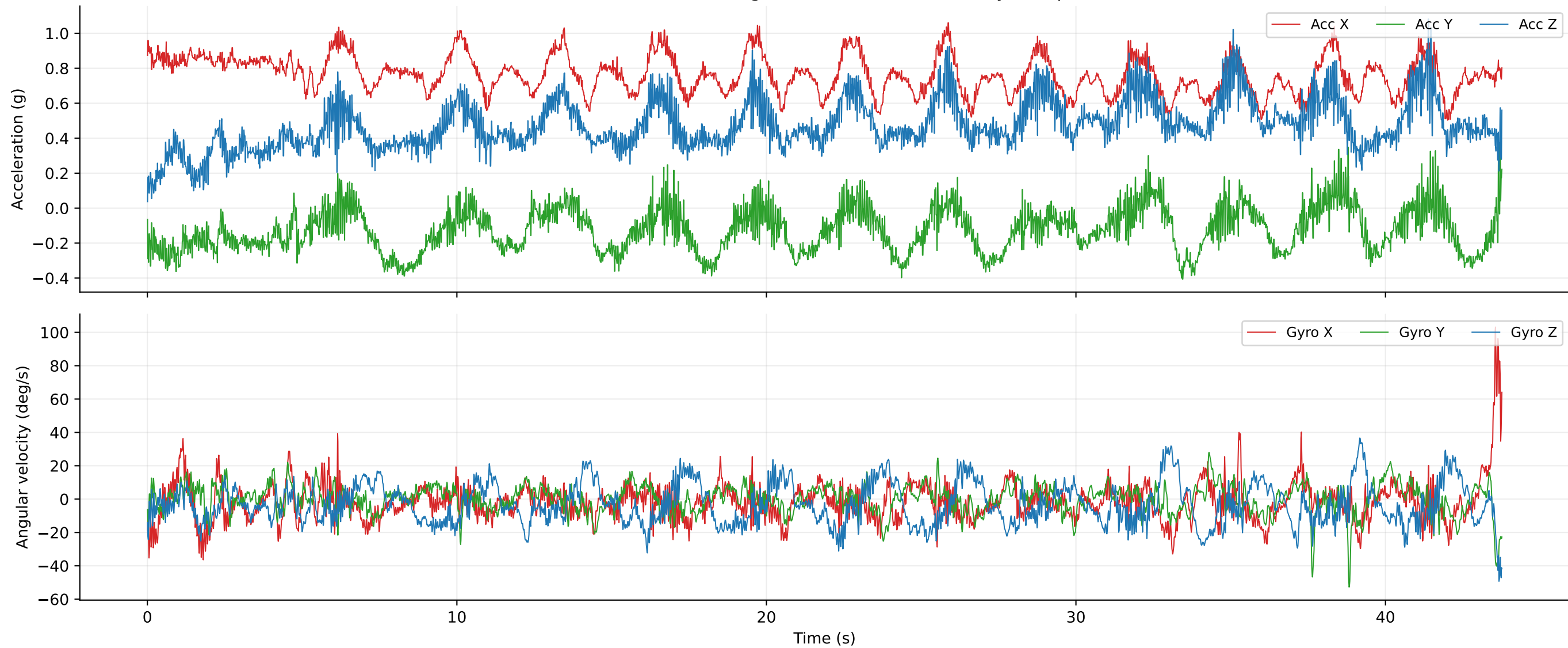
Six-Axis IMU Raw Signal: Accelerometer and Gyroscope
