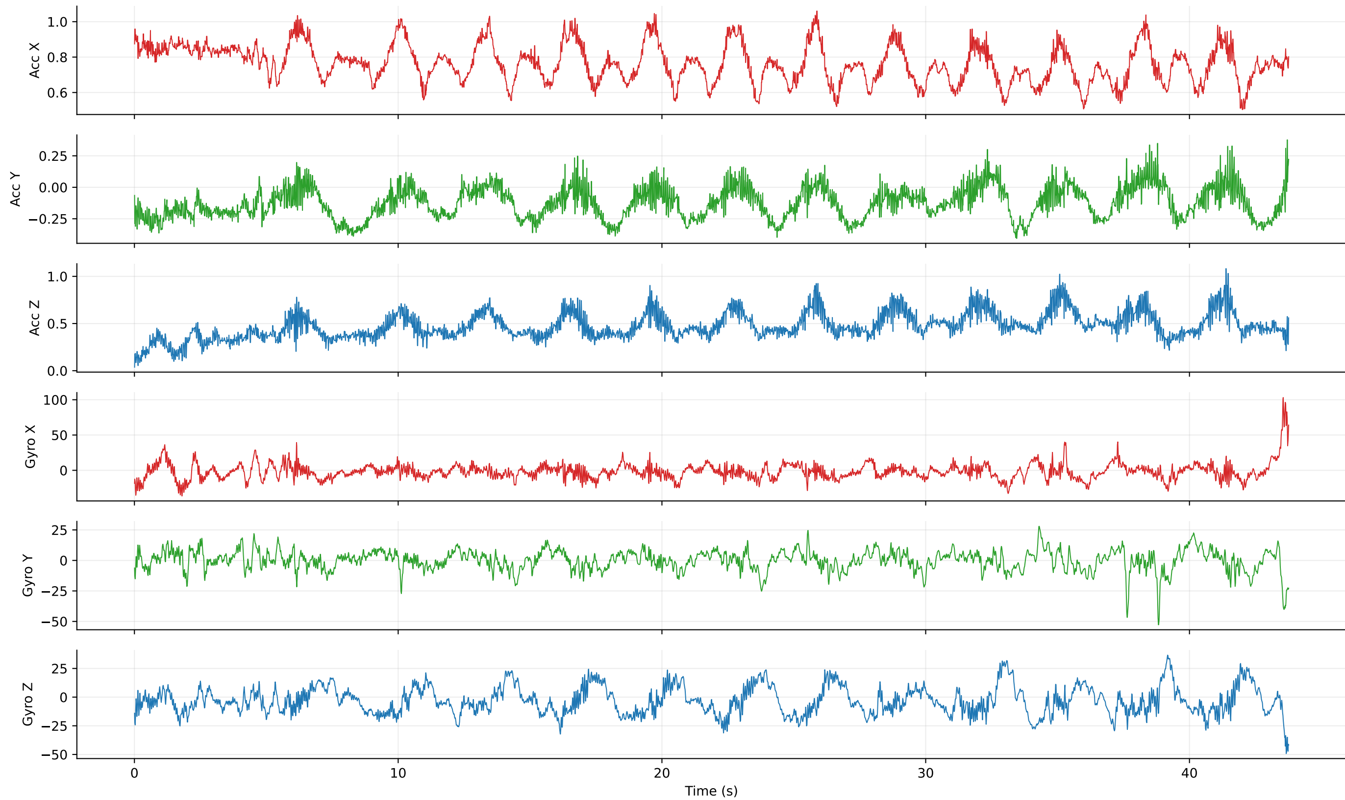
Six-Axis IMU Raw Waveforms
