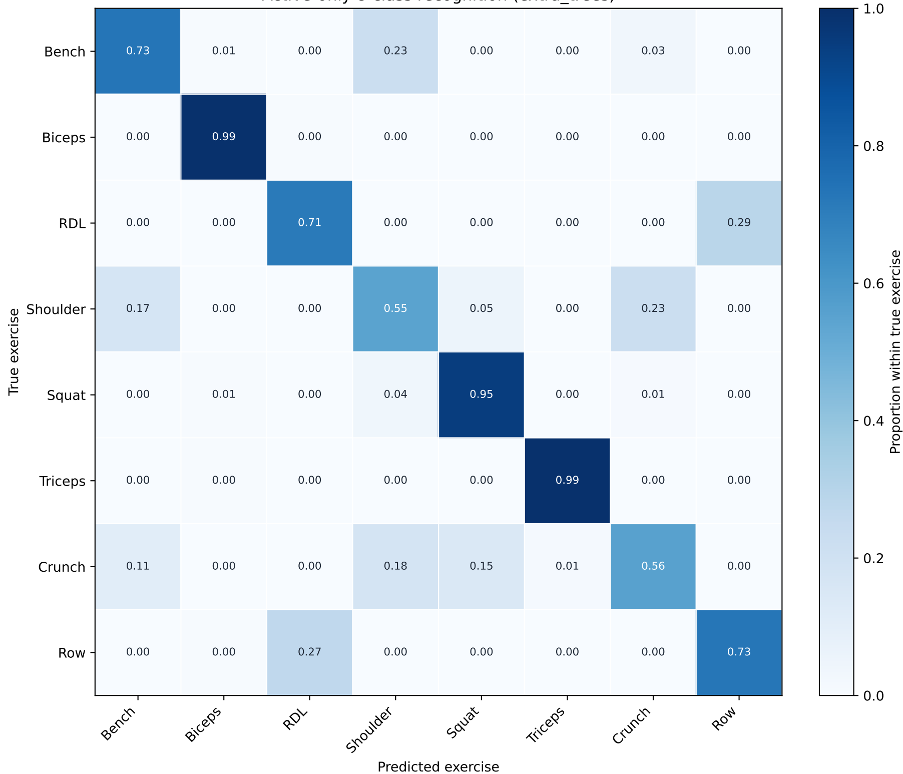
Active-only 8-class recognition (extra_trees)
