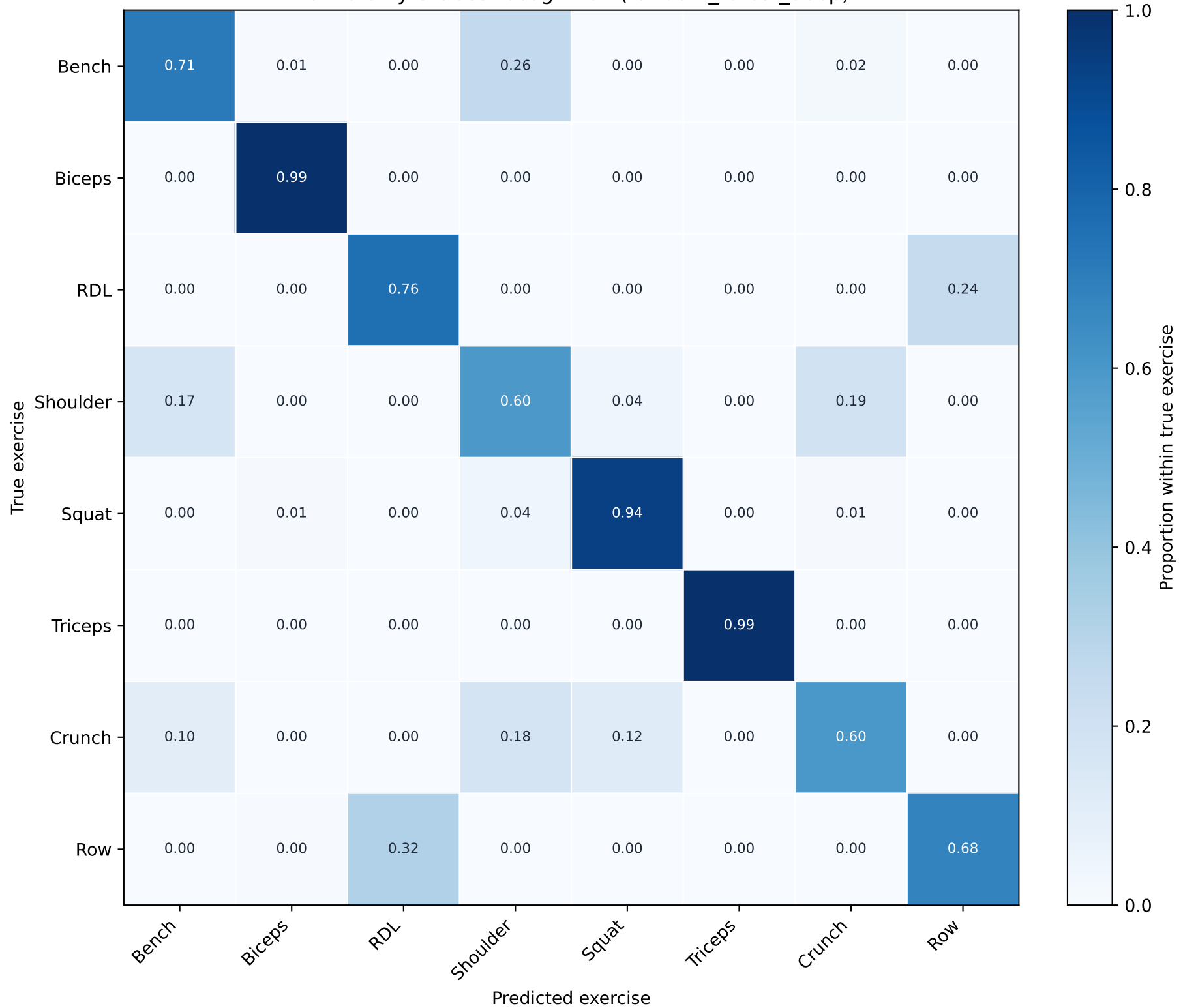
Active-only 8-class recognition (random_forest_deep)
