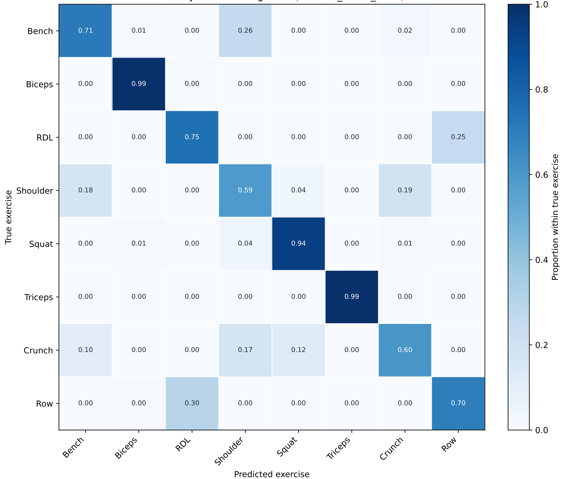
Active-only 8-class recognition (random_forest_leaf2)
