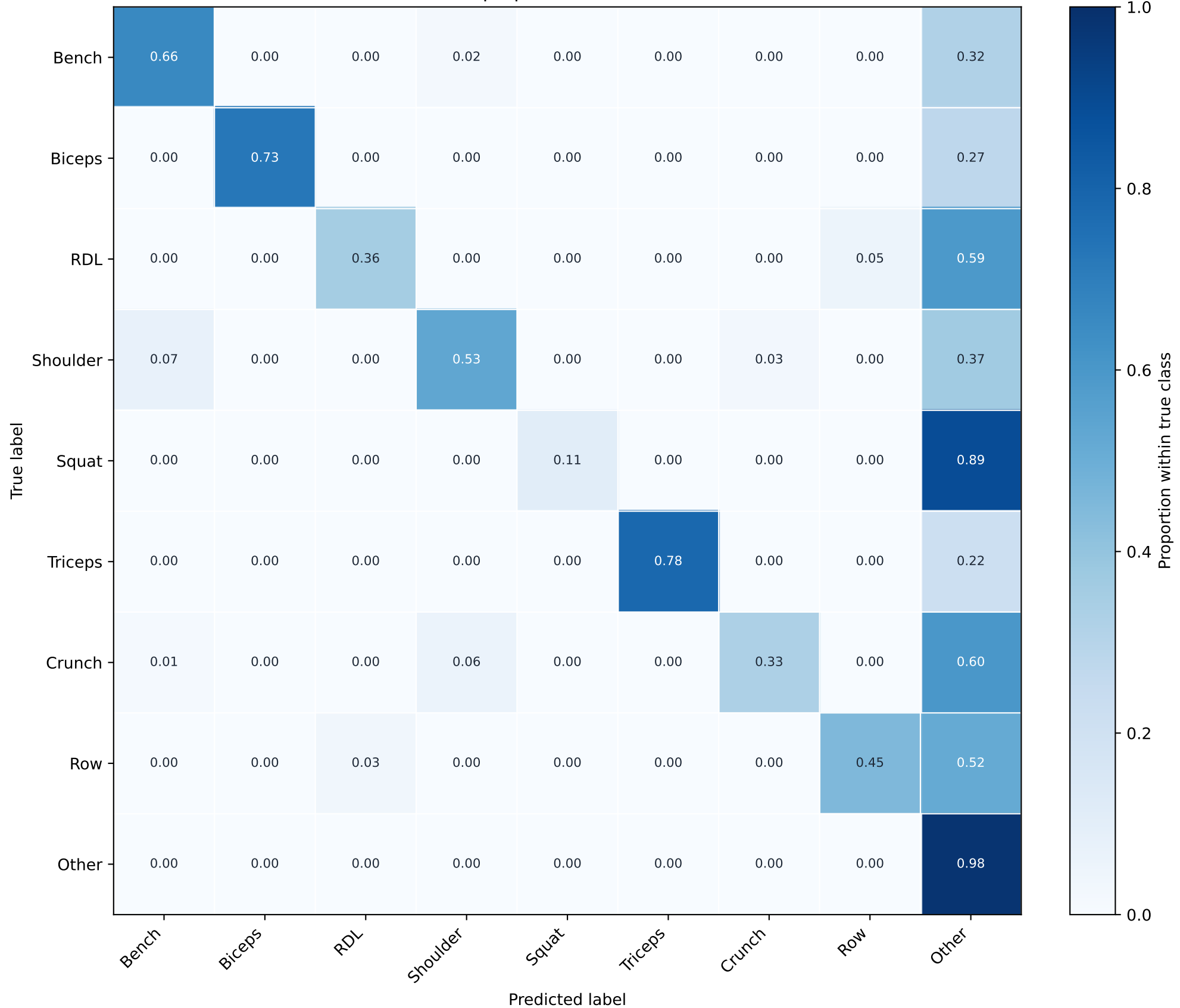
Realtime Action Recognition Confusion Matrix Row-normalized proportion, online smoothed k=11
