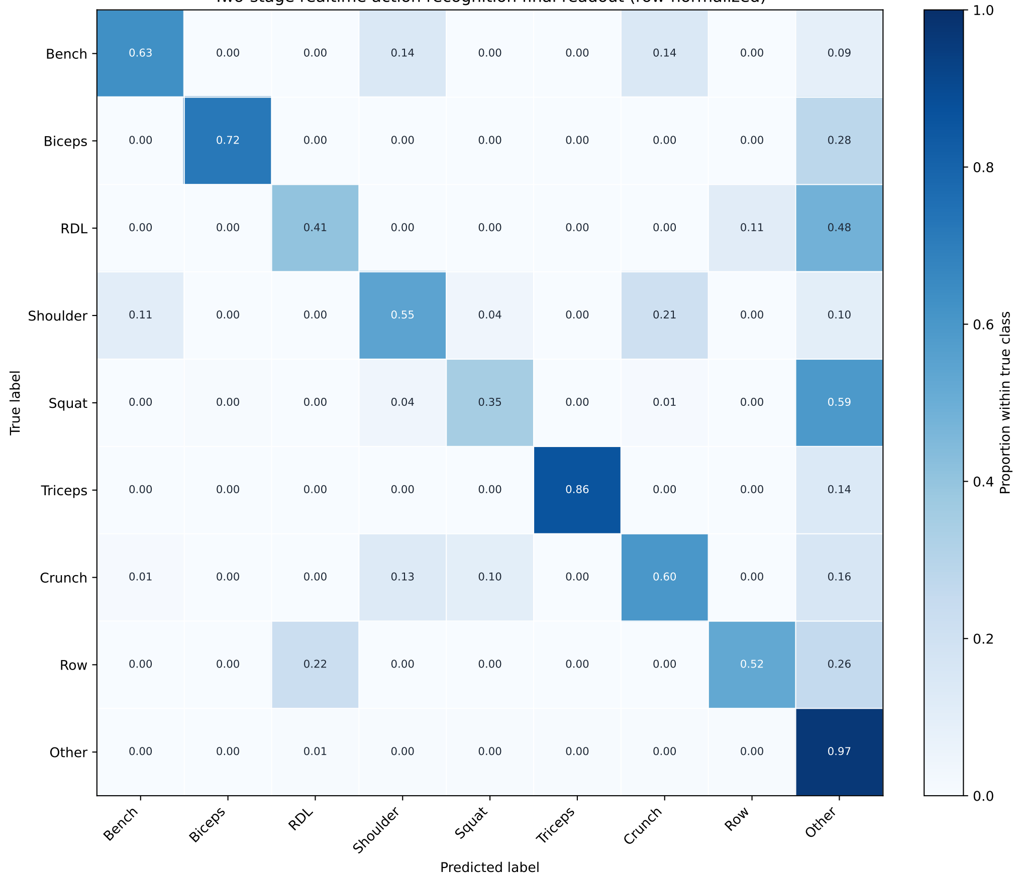
Two-stage realtime action recognition final readout (row-normalized)
