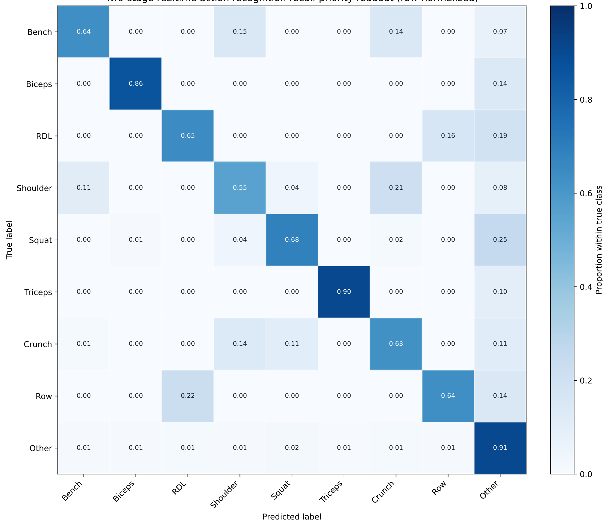
Two-stage realtime action recognition recall-priority readout (row-normalized)
