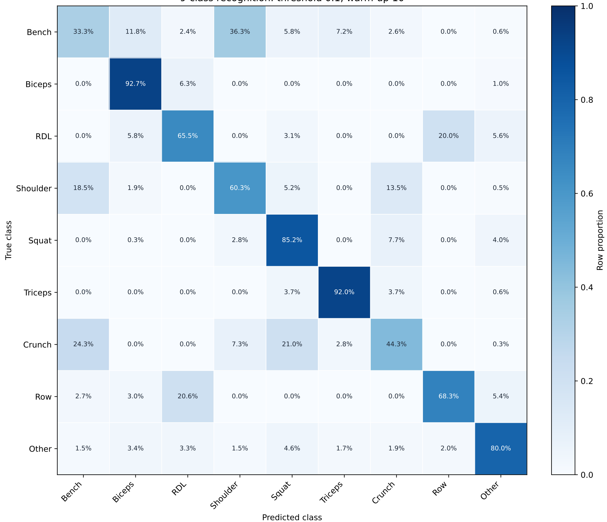
9-class recognition: threshold 0.1, warm-up 10
